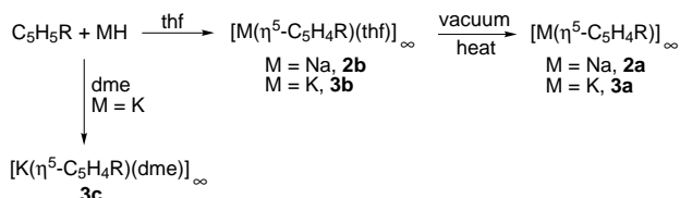
Scheme 2 dme = 1,2-Dimethoxyethane
